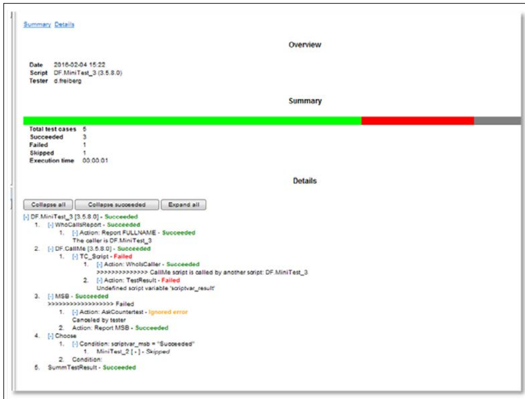
Figure 4: Automatically generated test report.
