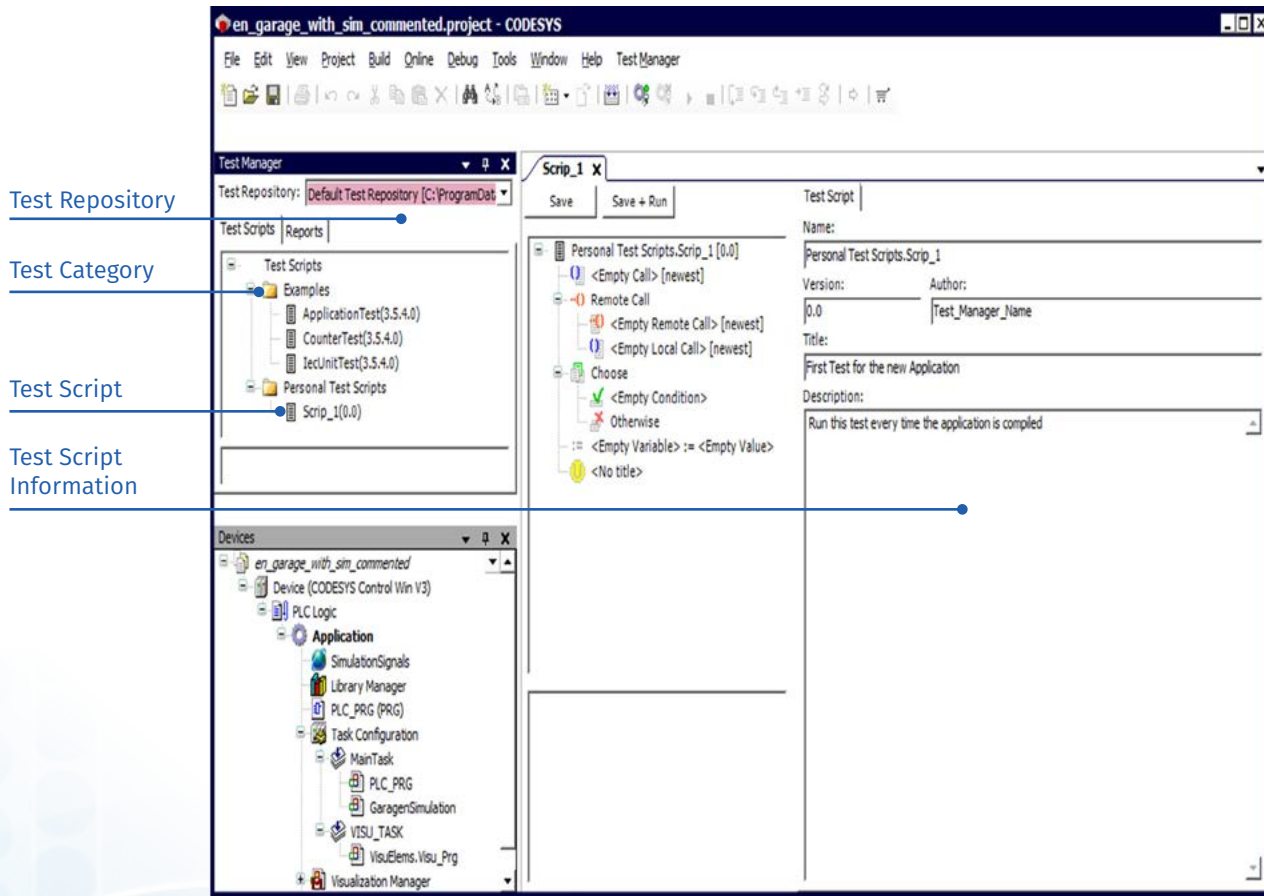
Figure 3: Overview of the CODESYS test manager in the IEC development environment.
