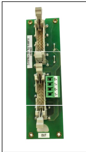
ANALOG OUTPUT PLC I/F ADAPTER PART #2302861
